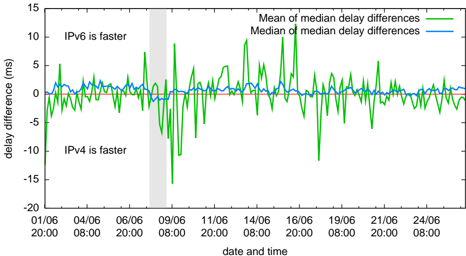
TCP connection setup delay differences (IPv4 - IPv6)
